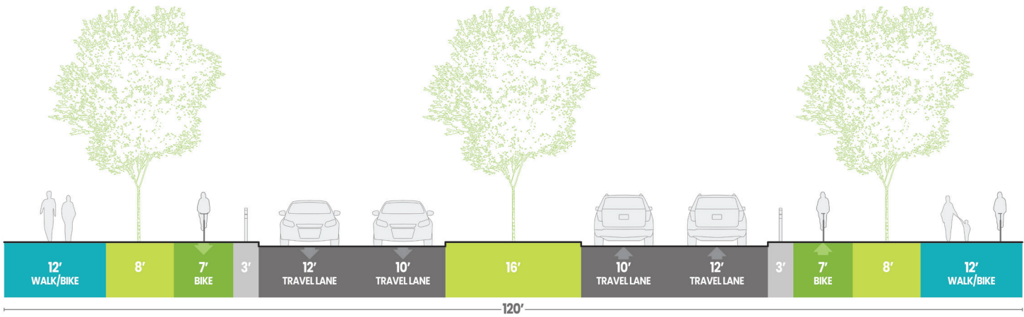
Major Arterial Separated Bikeway
