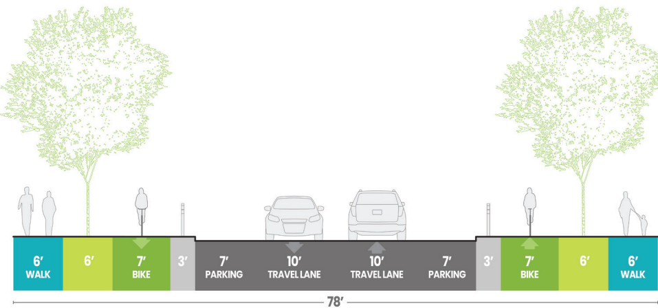
Collector Separated Bikeway with On-Street Parking
