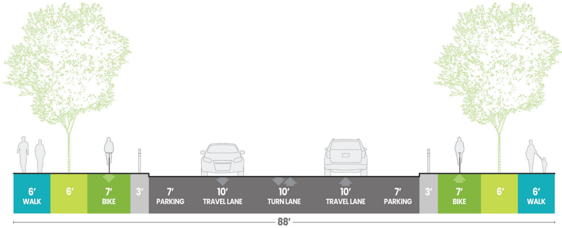
Minor Arterial Separated Bikeway with On-Street Parking
